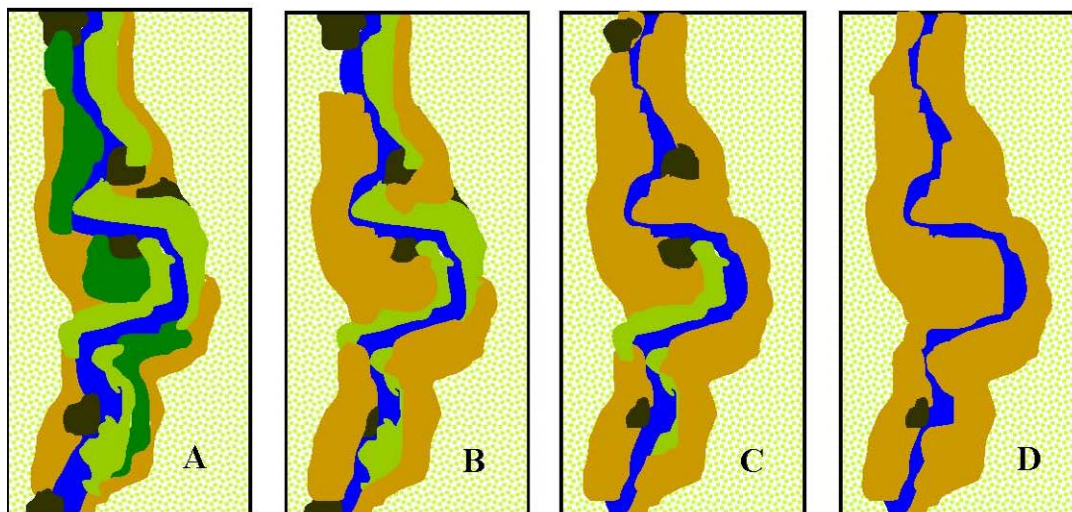
Figure 3. Schematic diagrams illustrating varying degrees of interspersed plant patches for riverine wetlands (from Collins et al. 2008).
